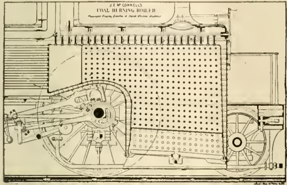
McCONNELL'S COAL BURNING FIRE BOX. FIG. 55.
